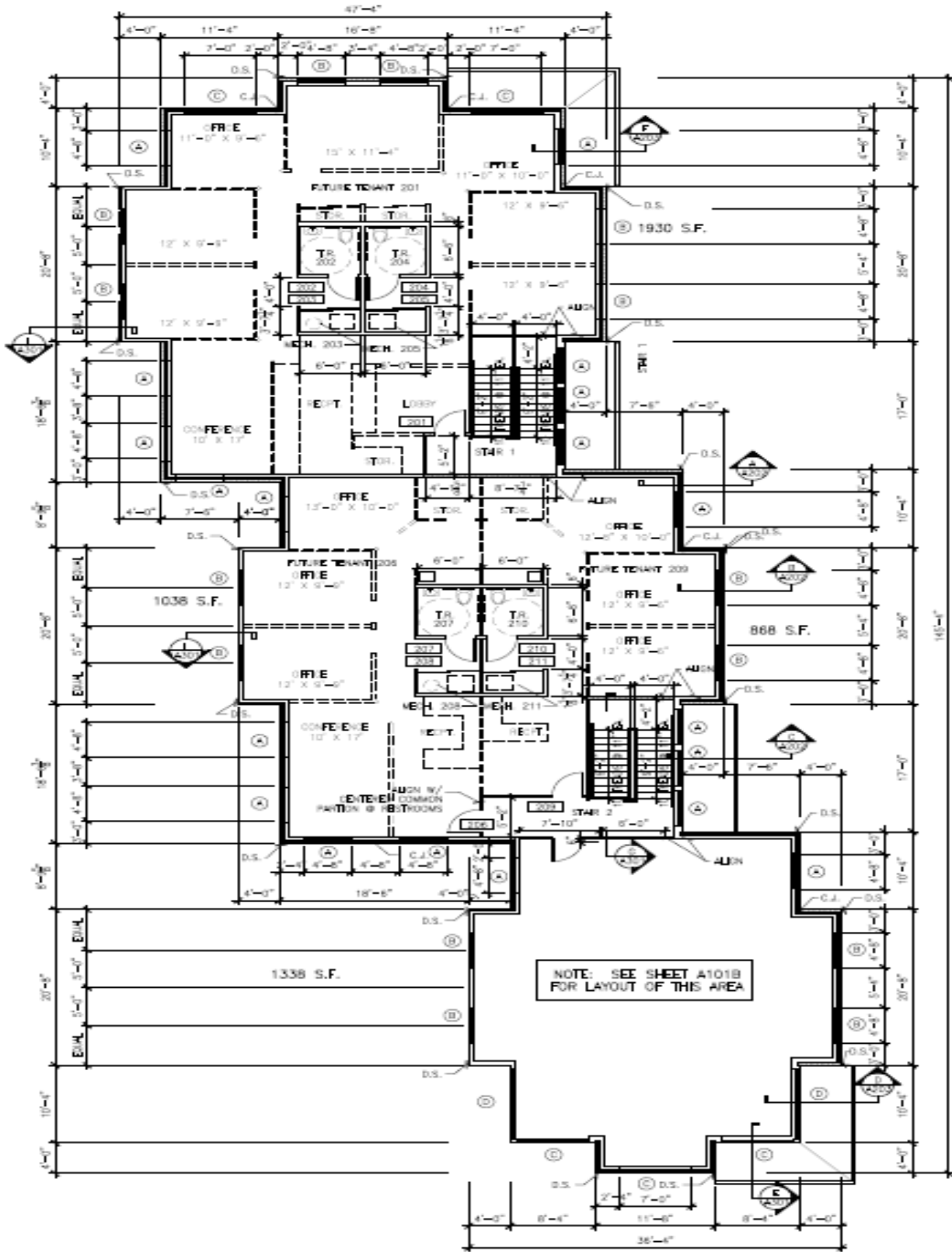
SECOND FLOOR NORTH 1/8" = 1'-0"
